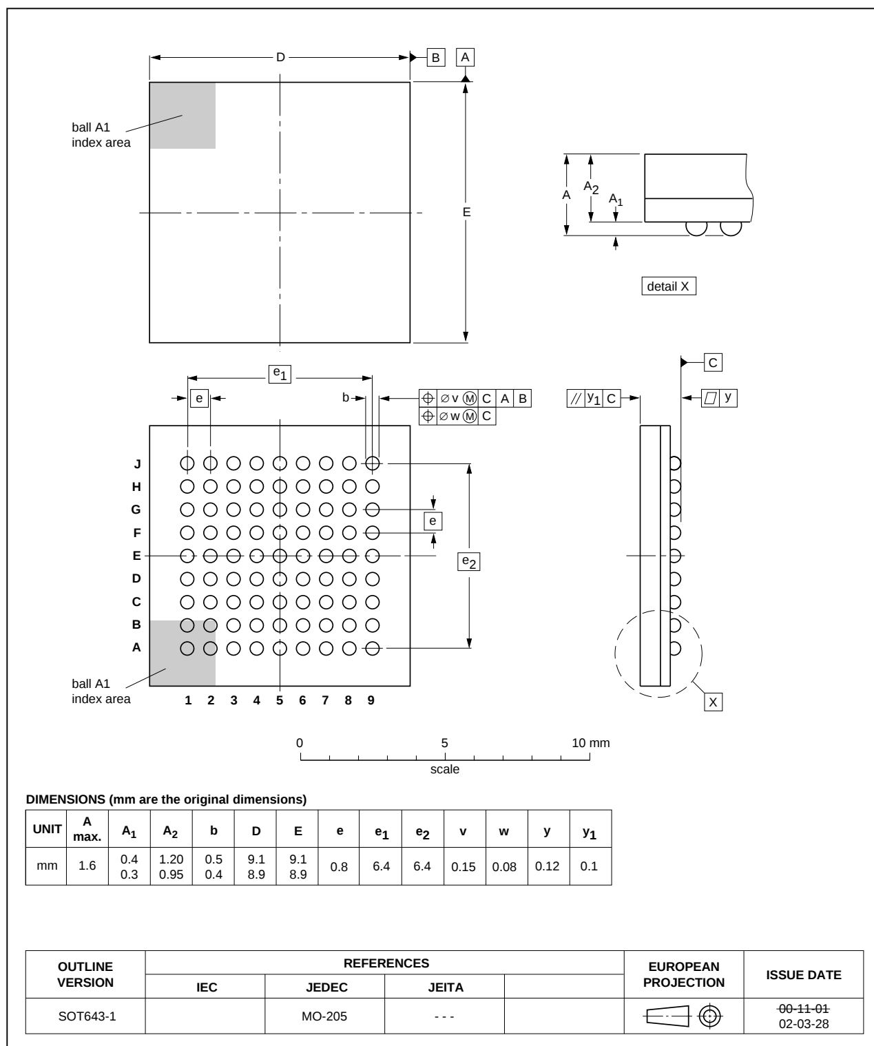
LFBGA81: plastic low profile fine-pitch ball grid array package; 81 balls; body 9 x 9 x 1.05 mm
