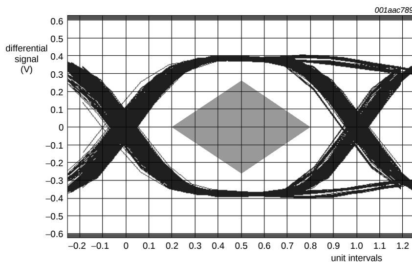
Fig 19. Transition eye
